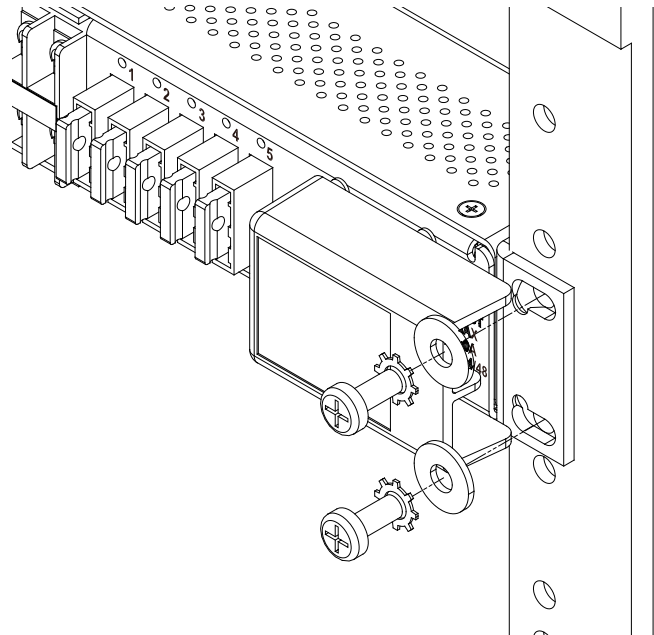
Figure 7 - Rack Mounting
