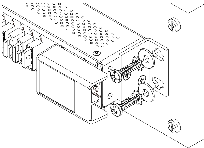
Figure 8 - Wall Mounting
